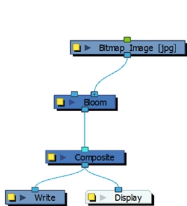
Basic Bloom node connection
