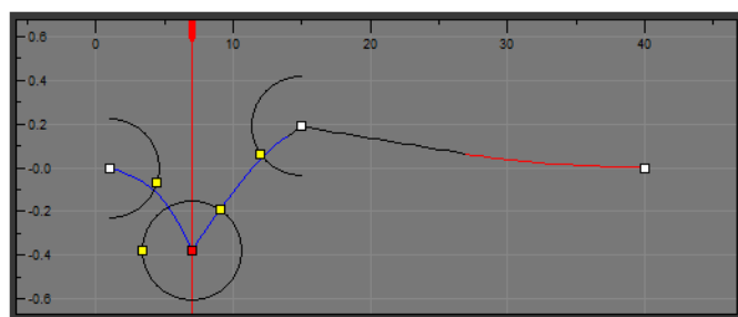
Ease function
