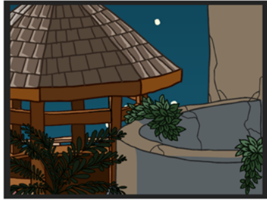
Orthographic camera
